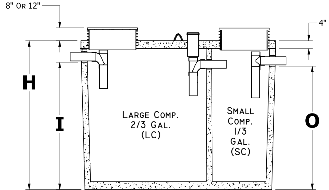
FRONT SECTIONAL VIEW
