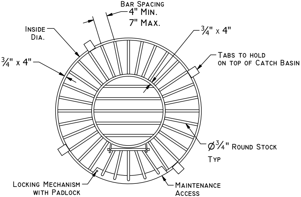
TOP VIEW
