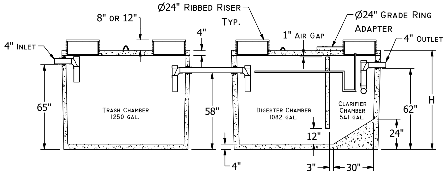
FRONT SECTIONAL VIEW
