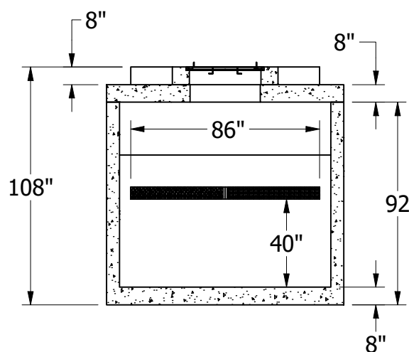
LEFT SECTIONAL VIEW SECTION B-B
