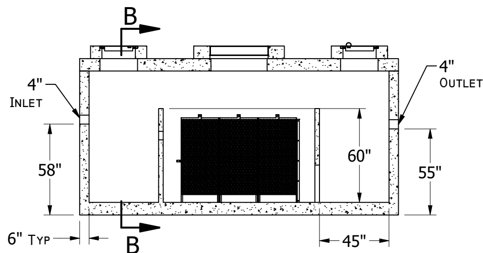
FRONT SECTIONAL VIEW
