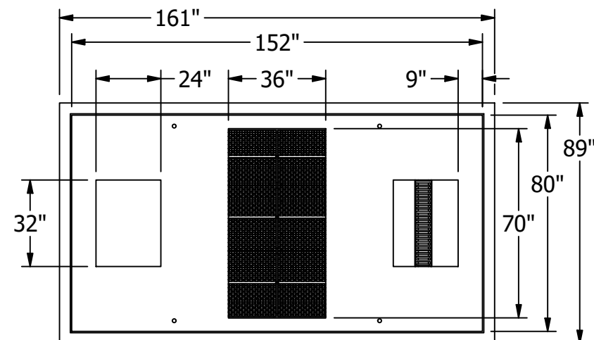
TOP VIEW HATCHES OMITTED FOR VISIBILITY
