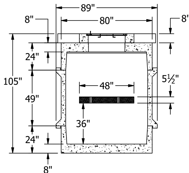
LEFT SECTIONAL VIEW SECTION A-A
