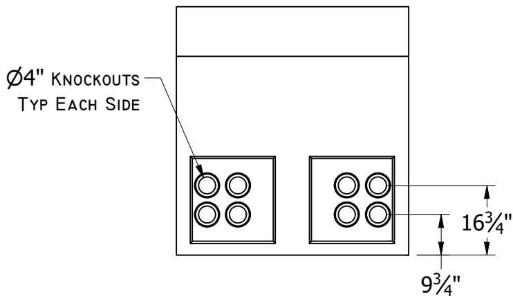
LEFT VIEW
