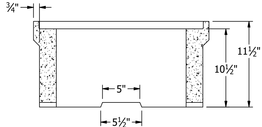
FRONT SECTIONAL VIEW
