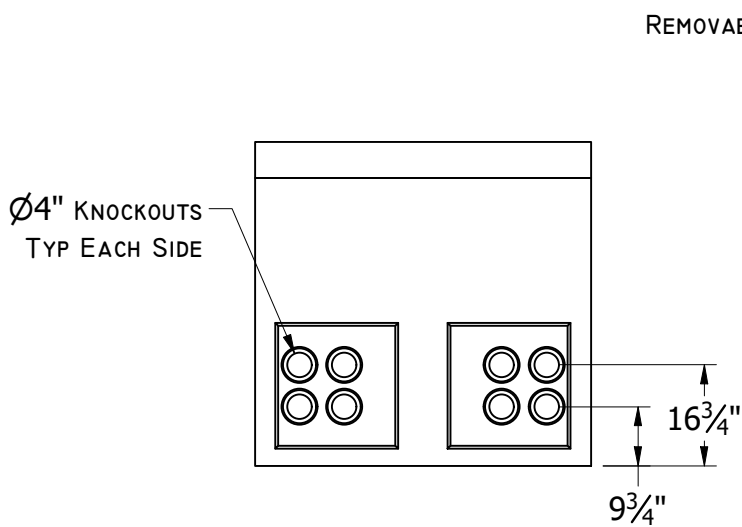
LEFT VIEW
