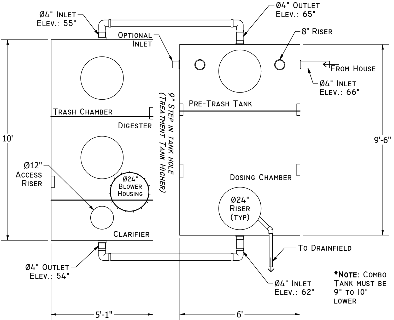
NU WATER COMBO (1500 GAL.)
