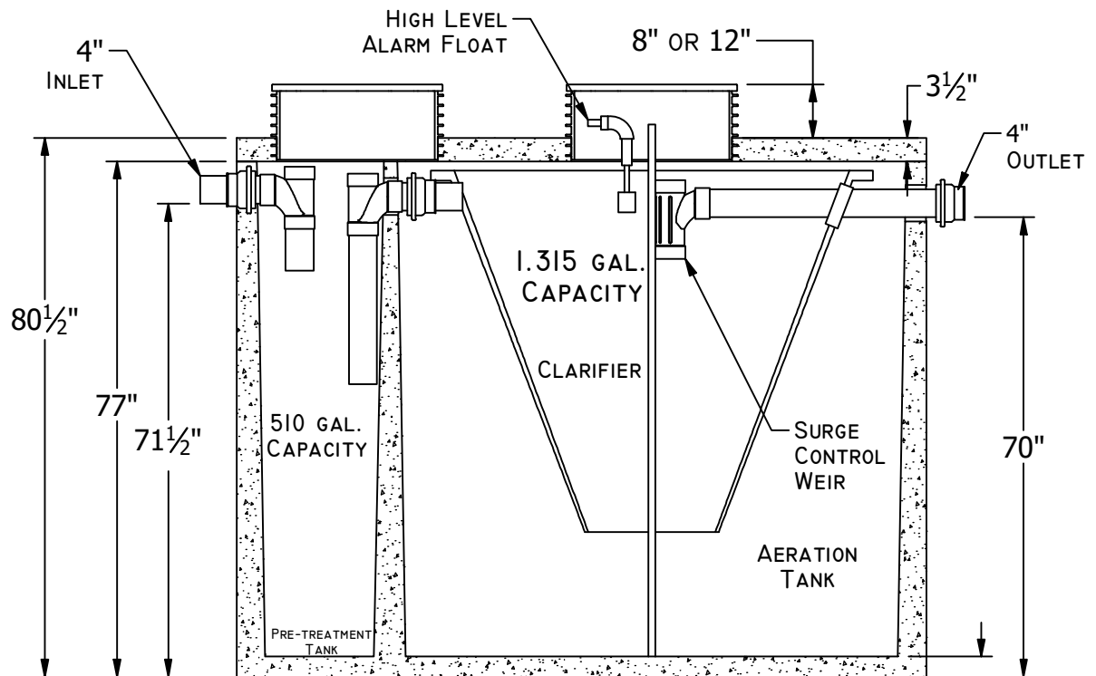
FRONT SECTIONAL VIEW
