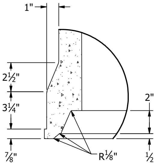
DETAIL C
