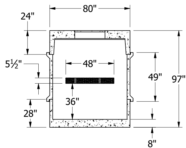
LEFT SECTIONAL VIEW SECTION F-F
