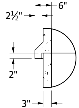
DETAIL H DIMENSIONS TYPICAL
