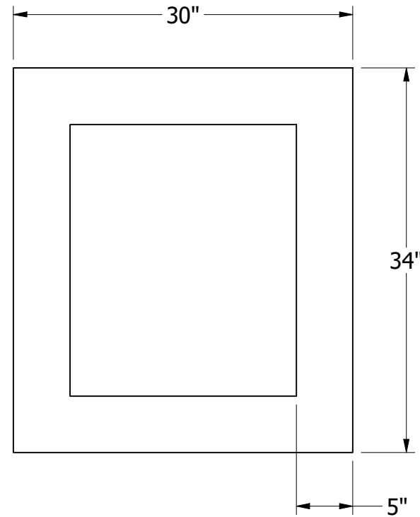
TOP VIEW
