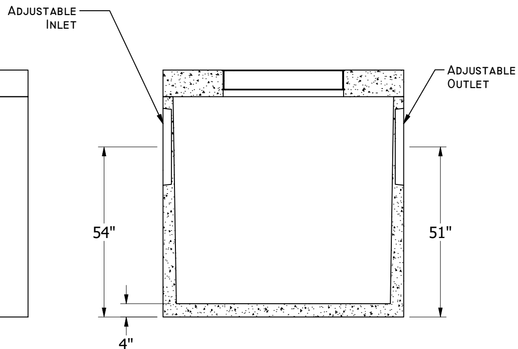
FRONT SECTIONAL VIEW
