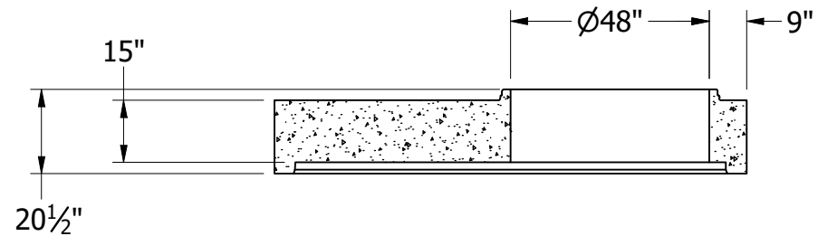
FRONT SECTIONAL VIEW
