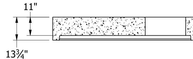
FRONT SECTIONAL VIEW
