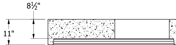
FRONT SECTIONAL VIEW
