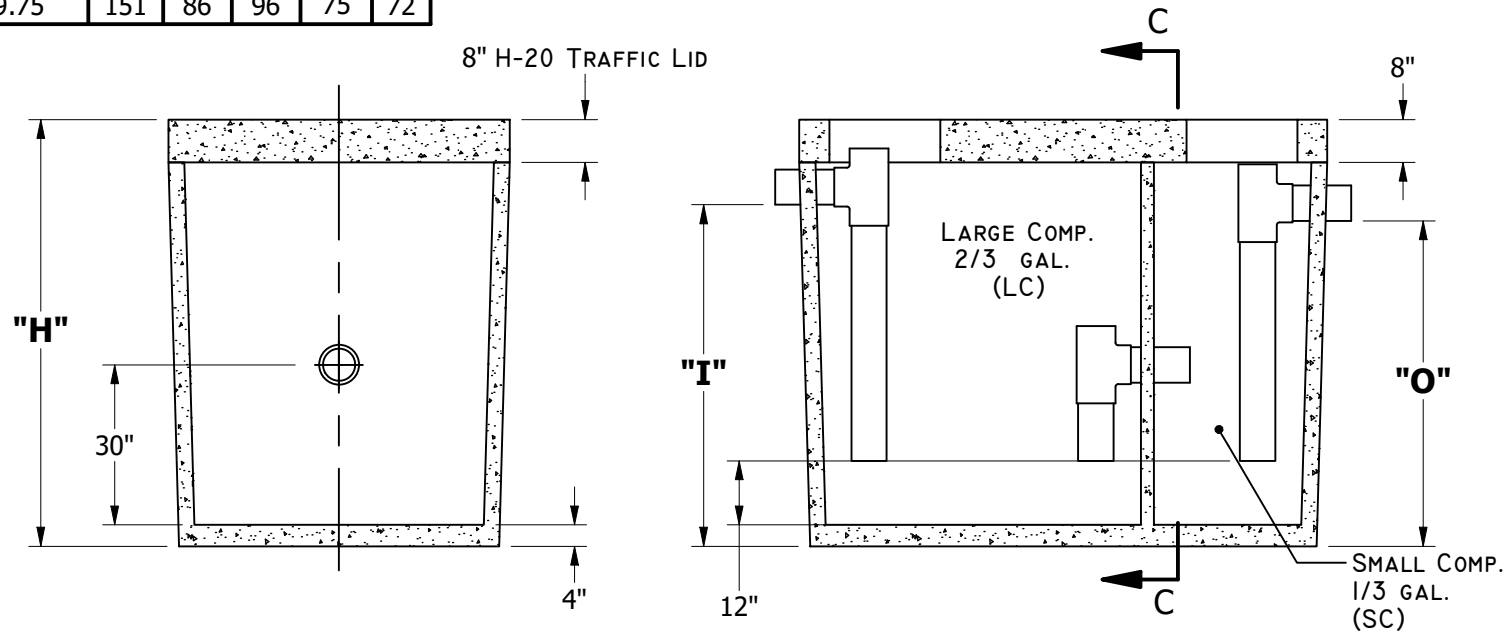
LEFT SECTIONAL VIEW
