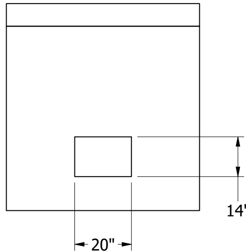
LEFT VIEW
