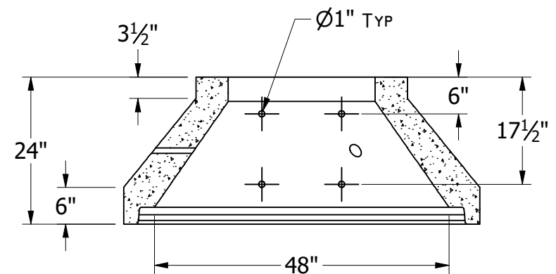
FRONT SECTIONAL VIEW
