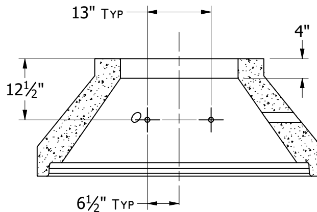
BACK SECTIONAL VIEW
