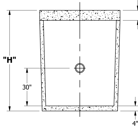
RIGHT SECTIONAL VIEW SECTION C-C
