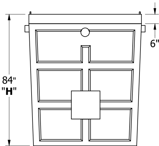
RIGHT VIEW
