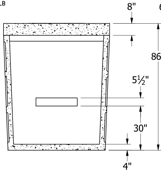
RIGHT SECTIONAL VIEW SECTION B-B
